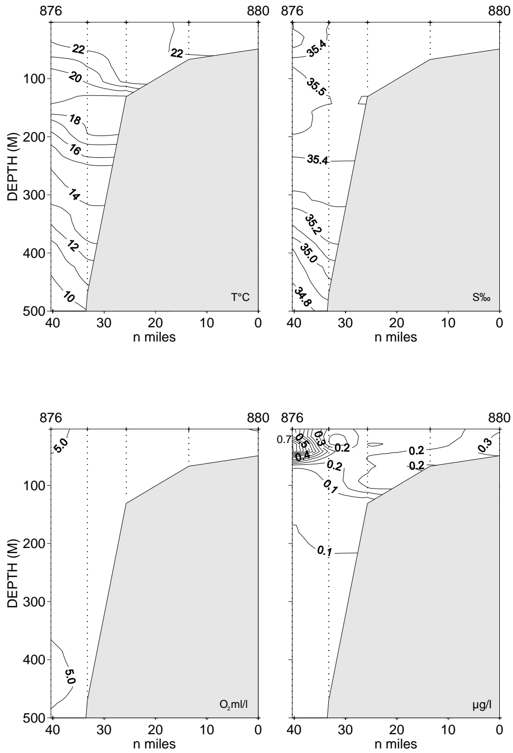
Fig. 3.5. Vertical sections of temperature, salinity, oxygen and fluorescence
