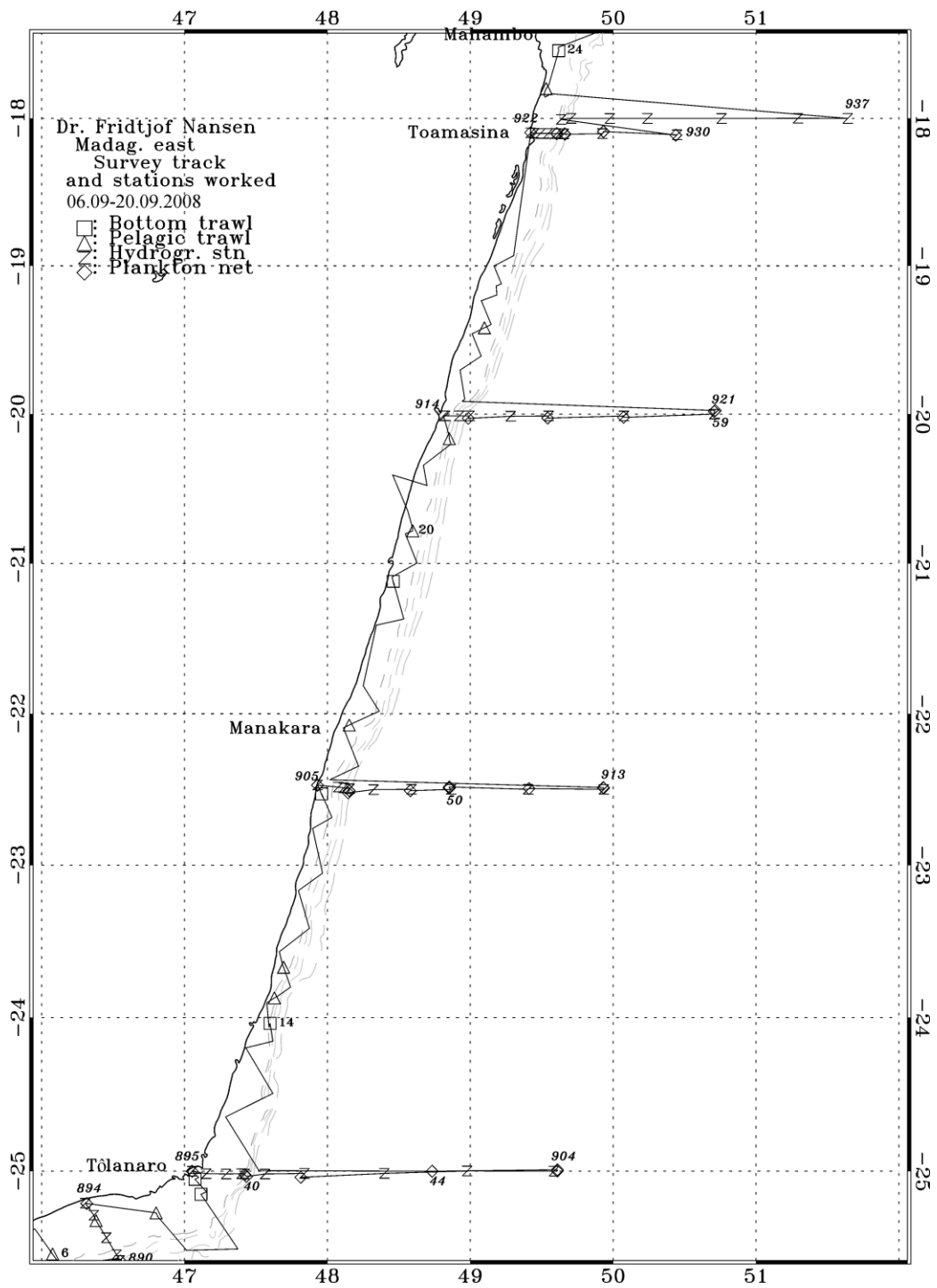
Figure 1.2. South-eastern coast. Course tracks with bottom trawl, pelagic trawl, plankton, and hydrographic stations. The 100, 500 and 1000 m depth contours are indicated.
