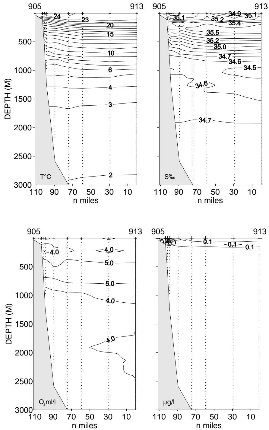
Fig. 3.10. Vertical sections of temperature, salinity, oxygen and fluorescence
