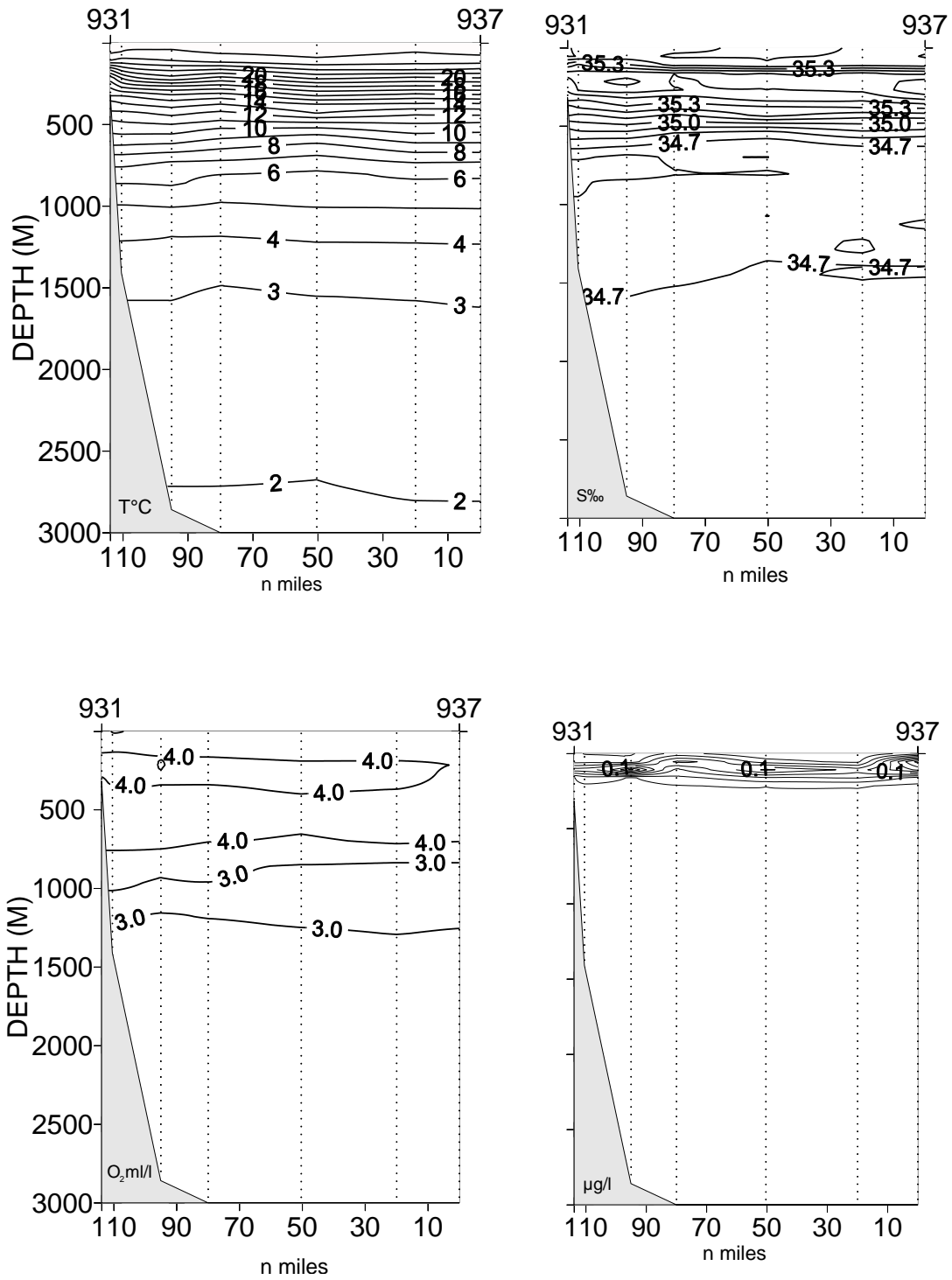
Fig. 3.13. Vertical sections of temperature, salinity, oxygen and fluorescence
