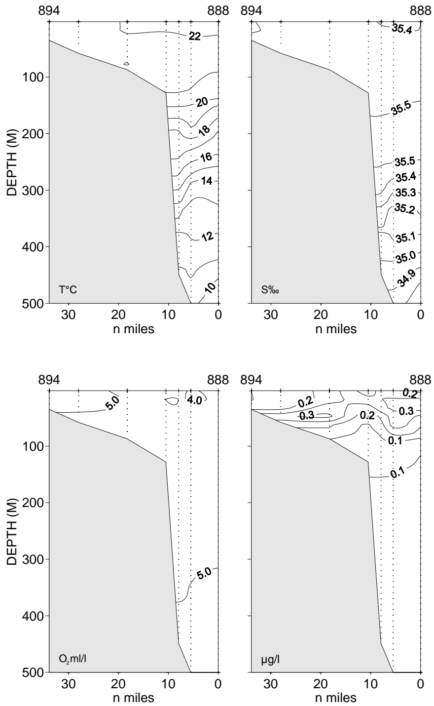
Fig. 3.7. Vertical sections of temperature, salinity, oxygen and fluorescence
