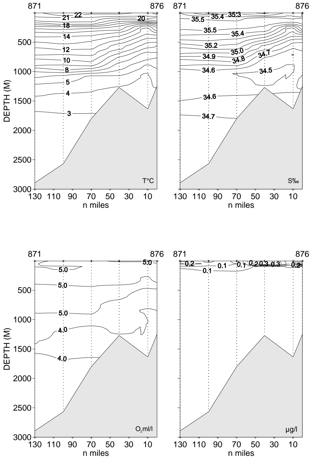
Fig. 3.4. Vertical sections of temperature, salinity, oxygen and fluorescence
