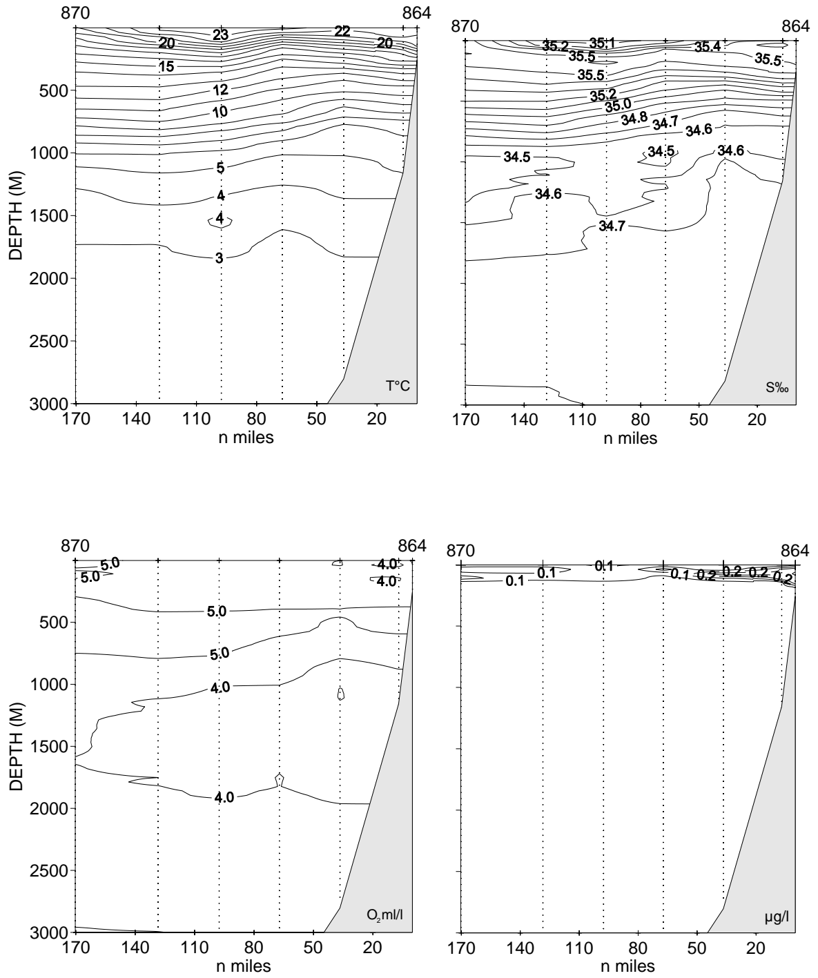
Fig. 3.3. Vertical sections of temperature, salinity, oxygen and fluorescence
