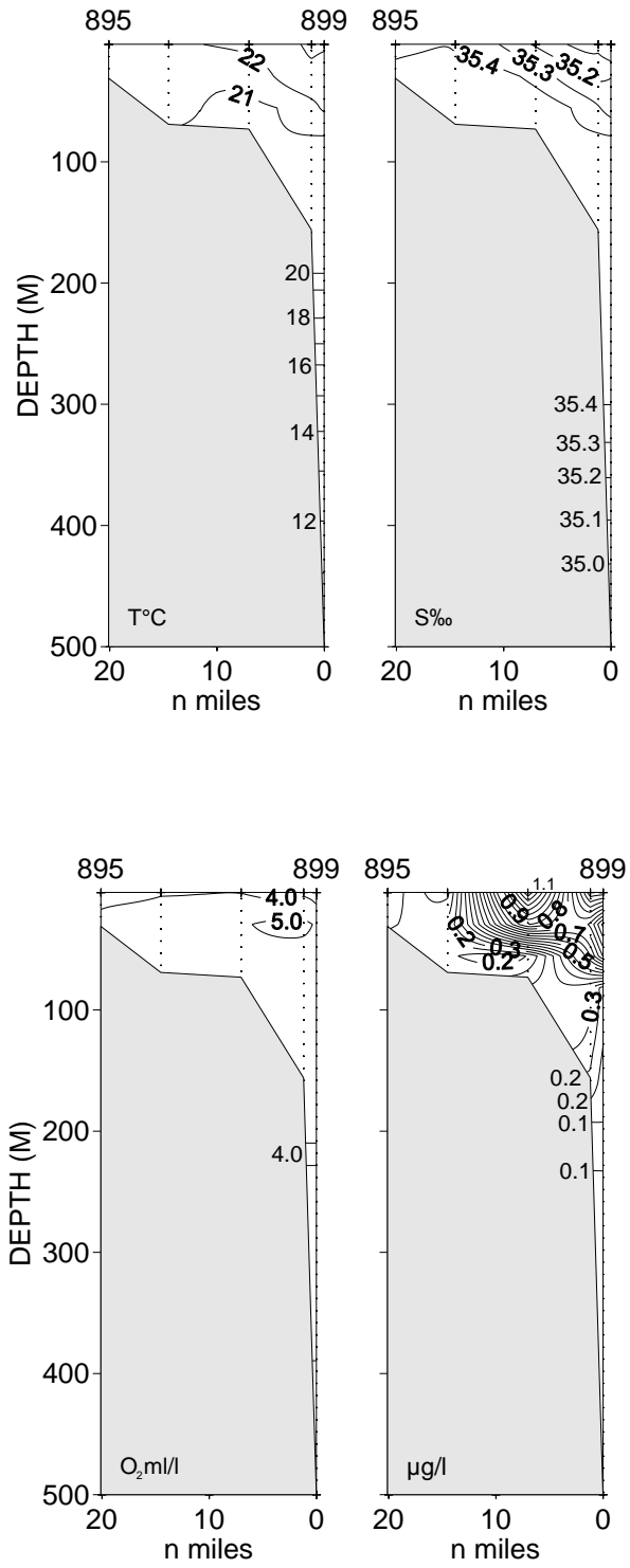
Fig. 3.9. Vertical sections of temperature, salinity, oxygen and fluorescence
