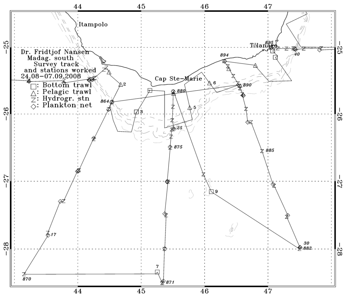
Figure 1.1. Southern region. Course tracks with bottom trawl, pelagic trawl, plankton and hydrographic stations. The 100, 500 and 1000 m depth contours are indicated.
