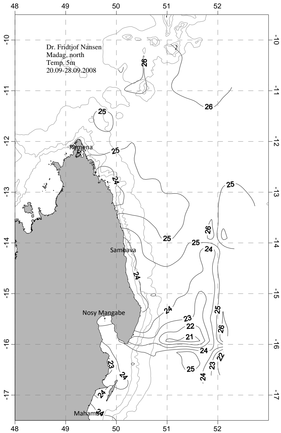
Figure 3.19 Horizontal distribution of sea temperature at 5 m on the north-eastern shelf of Madagascar based on data recorded underway. The 200, 1000 and 3000 m depth contours are indicated.
