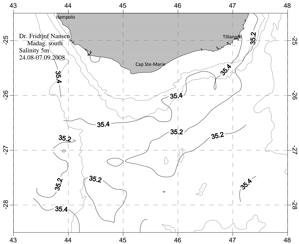
Figure 3.20 Horizontal distribution of salinity at 5 m on the Southern shelf of Madagascar based on data recorded underway. The 100, 1000 and 3000 m depth contours are indicated.
