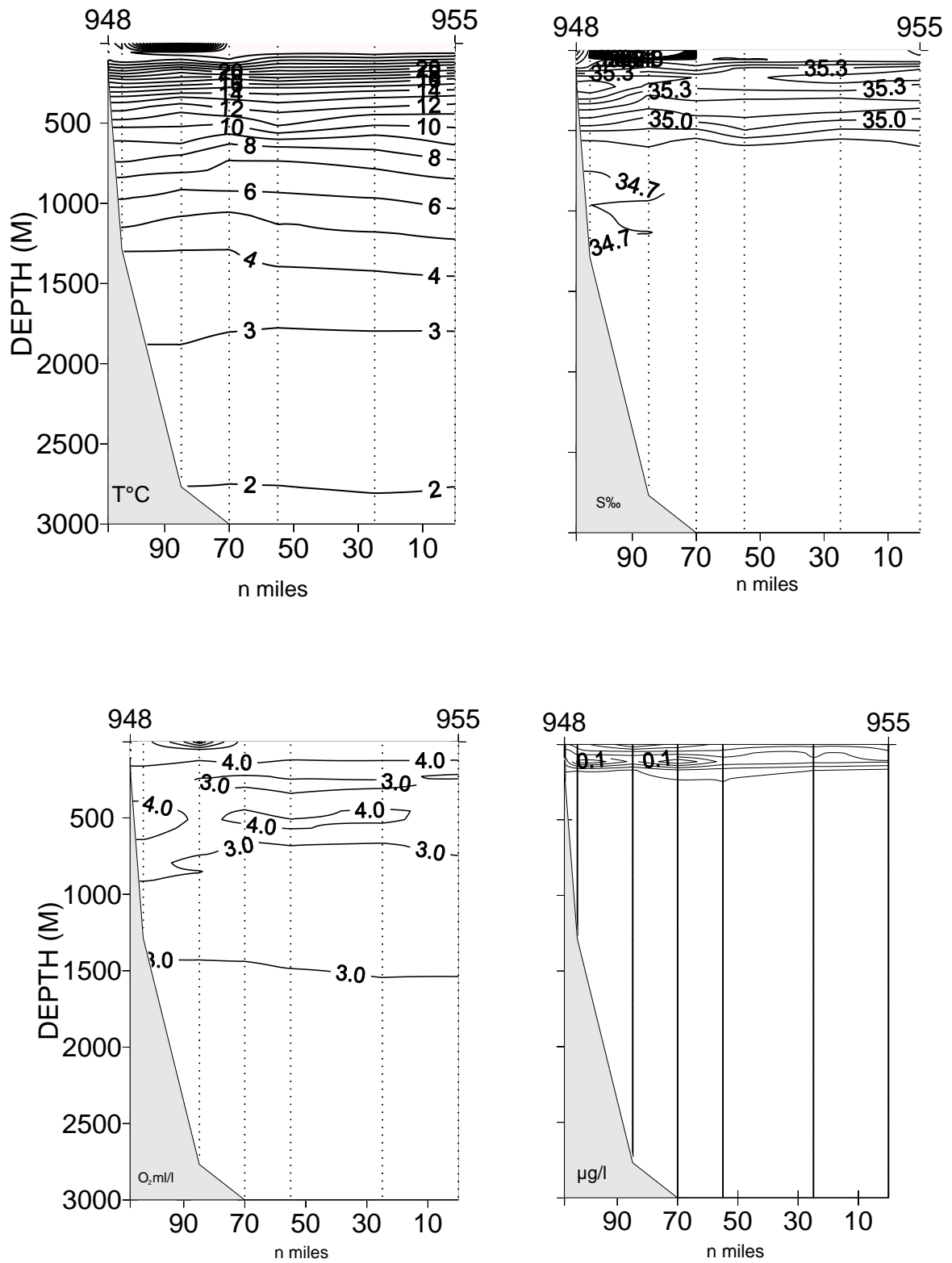
Fig. 3.15. Vertical sections of temperature, salinity, oxygen and fluorescence
