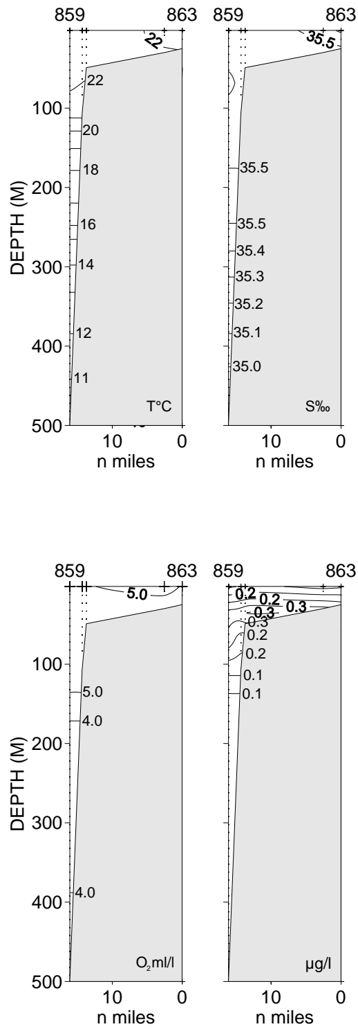
Fig. 3.2. Vertical sections of temperature, salinity, oxygen and fluorescence
