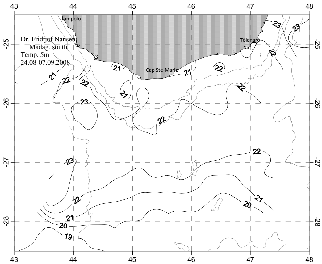
Figure 3.17 Horizontal distribution of sea temperature at 5 m on the Southern shelf of Madagascar based on data recorded underway. The 100, 1000 and 3000 m depth contours are indicated.
