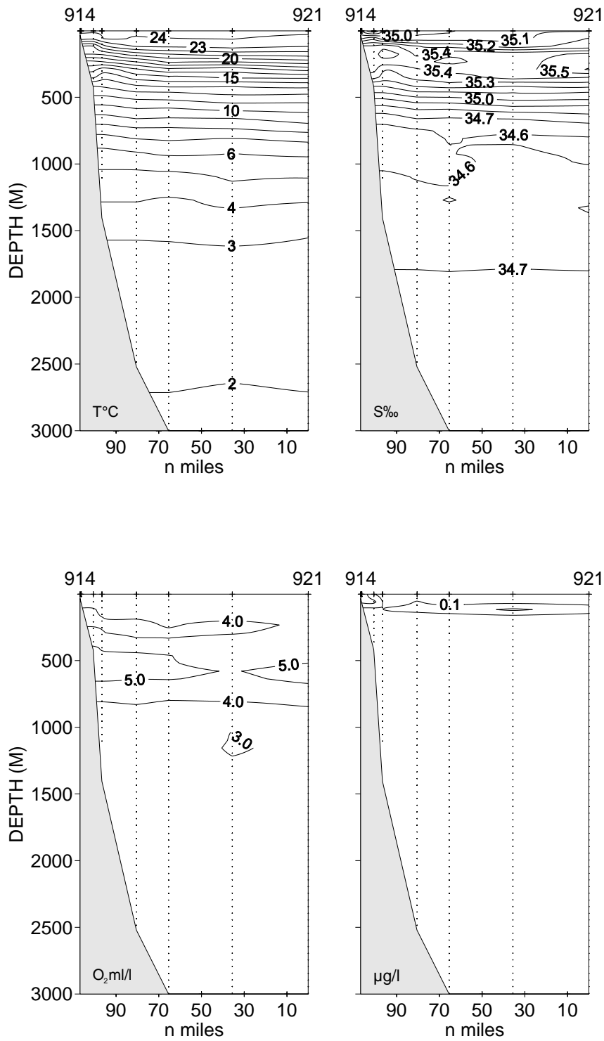
Fig. 3.11. Vertical sections of temperature, salinity, oxygen and fluorescence
