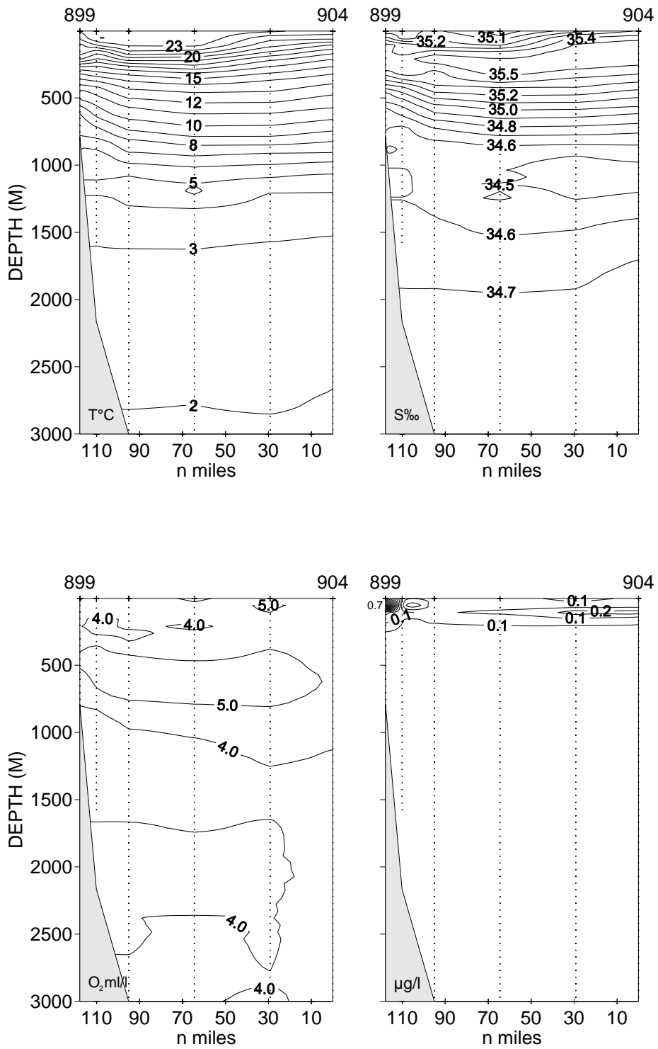
Fig. 3.8. Vertical sections of temperature, salinity, oxygen and fluorescence
