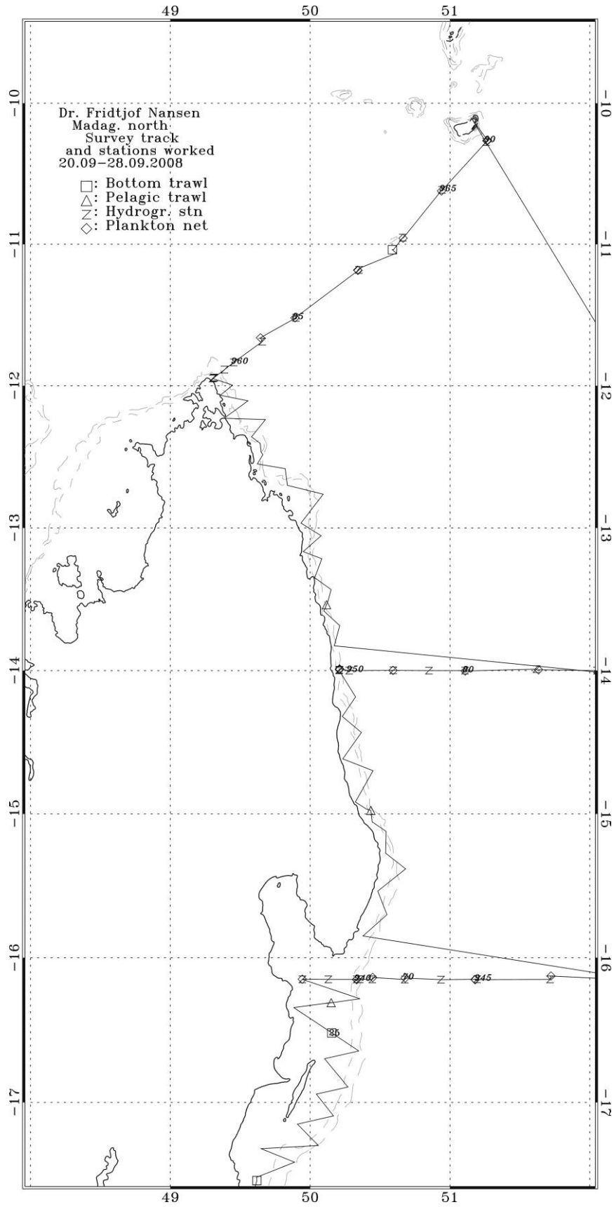
Figure 1.3. North-eastern coast and the Farquhar Group. Course tracks with bottom trawl, pelagic trawl, plankton, and hydrographic stations. The 100, 500 and 1000 m depth contours are indicated.
