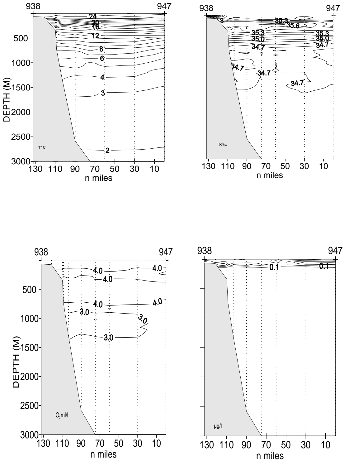
Fig. 3.14. Vertical sections of temperature, salinity, oxygen and fluorescence
