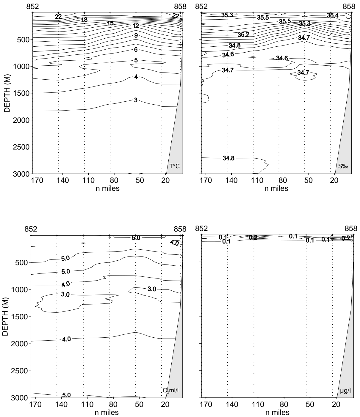
Fig. 3.1. Vertical sections of temperature, salinity, oxygen and fluorescence
