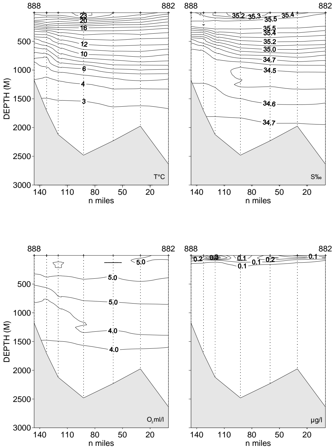
Fig. 3.6. Vertical sections of temperature, salinity, oxygen and fluorescence
