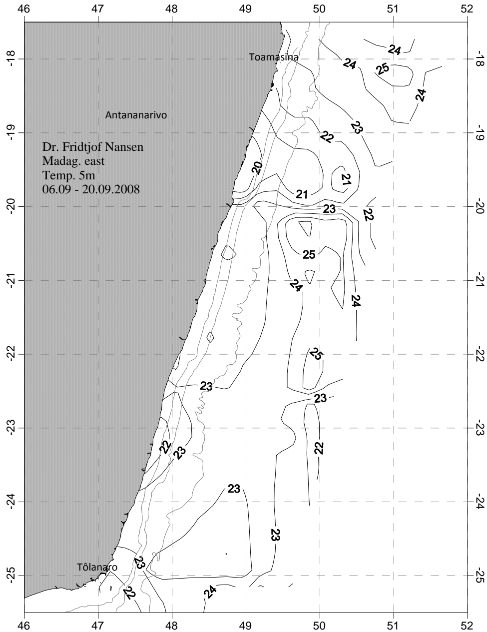
Figure 3.18 Horizontal distribution of sea temperature at 5 m on the south-eastern shelf of Madagascar based on data recorded underway. The 100, 1000 and 3000 m depth contours are indicated.
