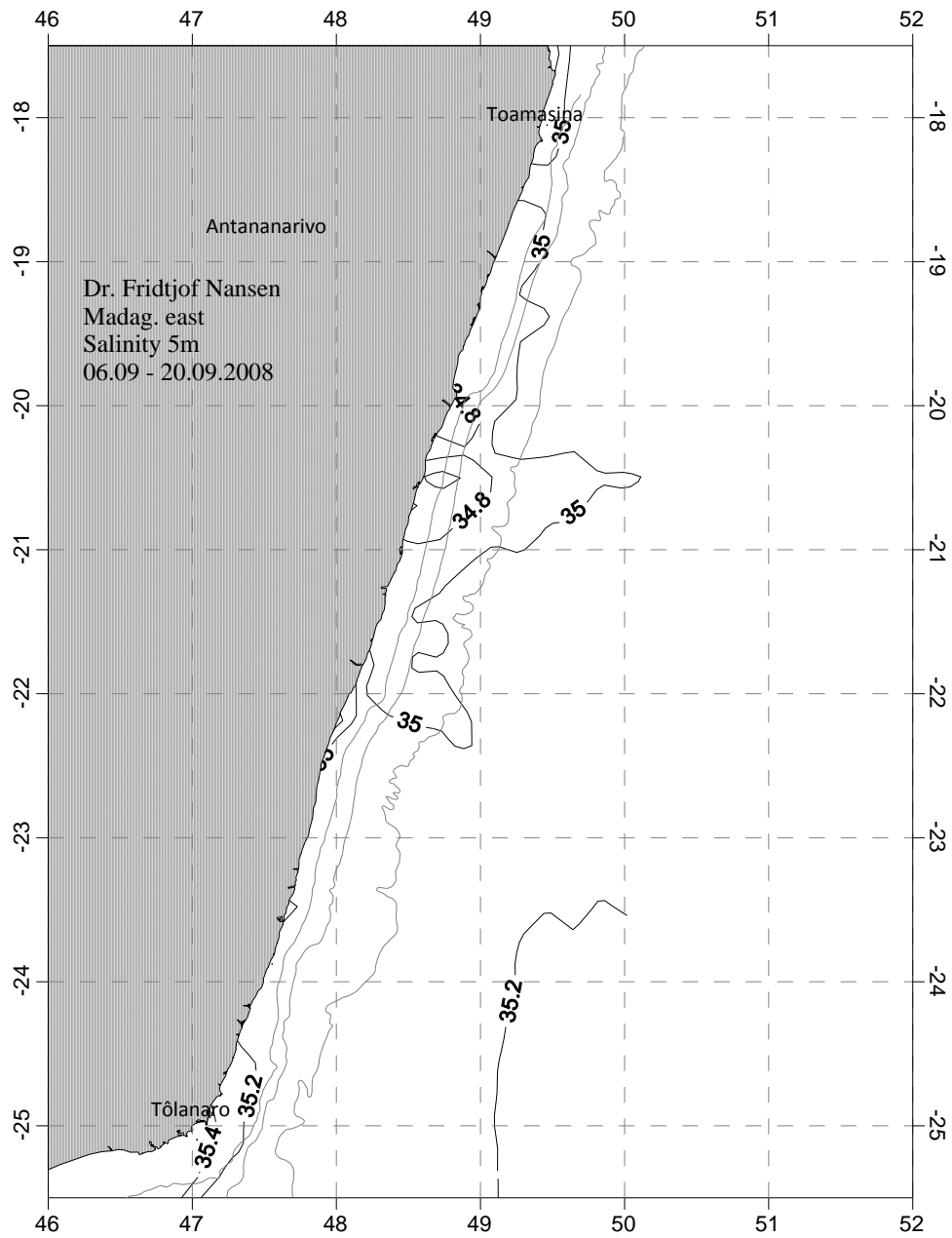
Figure 3.21 Horizontal distribution of salinity at 5 m on the south-eastern shelf of Madagascar based on data recorded underway. The 100, 1000 and 3000 m depth contours are indicated.
