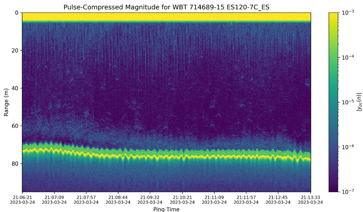
Figure 24: Example from T2023004 showing backscatter from individual capelin ( Mallotus villosus ) measured with the keel mounted echosounders of RV Johan Hjorth. The echogram shows data from the 120 kHz channel (95-165 kHz, frequency modulated up-sweep pulses, pulse-compressed) for about 7 minutes. The vertical axis to the left indicates the range (m) beneath the transducer. The color bar on the right represents the magnitude of the pulse-compressed signal. The bottom is seen at range around 75 m.
