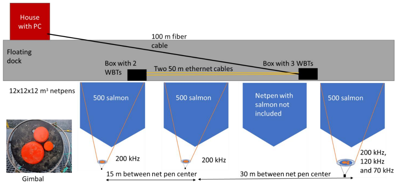
Figure 11: Experimental setup. Echosounder gimbals with 1-3 transducers under three net pens with 500 salmon at a floating dock attached to the shore in a fjord in western Norway. A netting at about 2 m depth was used to deprive salmon from access to the surface to simulate a submerged net pen where the air supply has failed.
