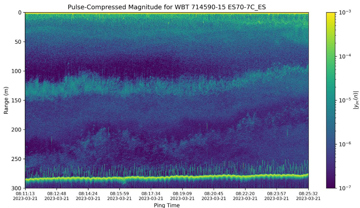
Figure 21: Example from T2023001 showing layers of fish and northern krill measured with keel mounted echosounders from RV G.O. Sars. The echogram shows about 14 minutes of data from the 70 kHz channel (50-85 kHz, frequency modulated up-sweep pulses, pulse-compressed) The upper layer consisting of Atlantic herring ( Clupea harengus ), Atlantic mackerel ( Scomber scombrus ) and northern krill ( Meganyctiphanes norvegica ), the centre layer consisting of blue whiting ( Micromesistius poutassou ) and muellers pearlside ( Maurollicus muelleri ), the bottom layer was dominated by blue whiting. Noise from other instruments can be seen close to the bottom of the echogram for this channel. The vertical axis to the left indicates the range (m) beneath the transducer. The color bar on the right represents the magnitude of the pulse-compressed signal. The bottom is seen at range around 290 m.
