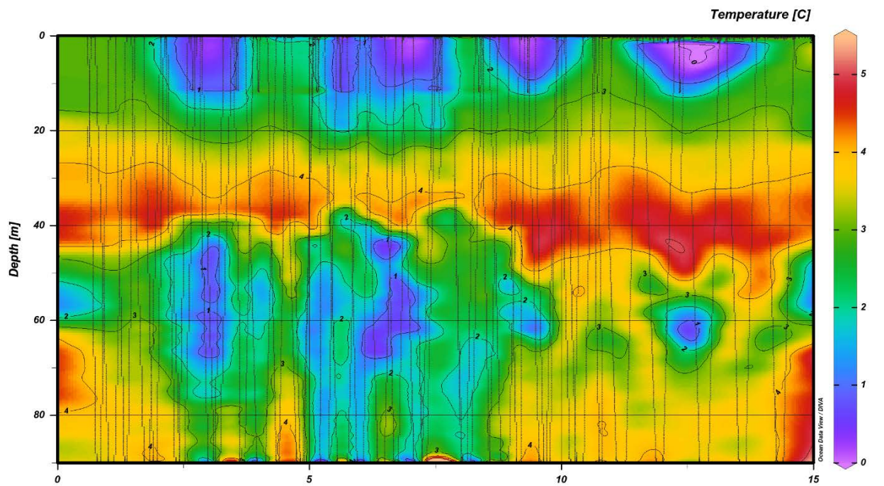
Figure 41: Temperature Profile from the TRES adaptive sampling mission. The AUV crosses back and forth from warm to cold waters.
