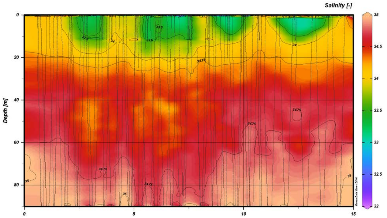
Figure 40: Salinity Profile from the TRES adaptive sampling mission. The AUV crosses back and forth from saline to fresher waters.
