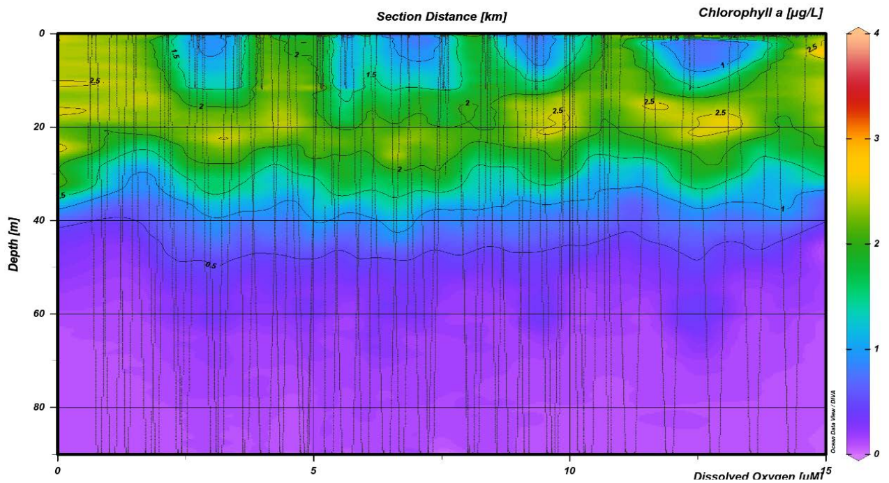
Figure 42: Chlorophyll profile from the TREX adaptive sampling mission. Higher values in shallow, as well as fresh waters.
