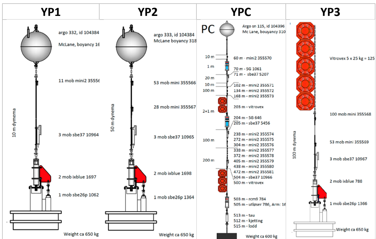
Figure 26: REOCIRC mooring design with instrument setup and deployment depth specifications.
