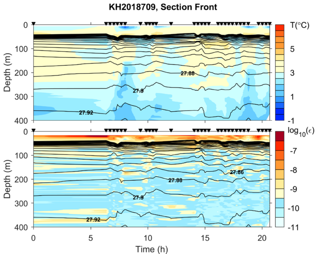
Figure 34. Process Station 1 (Front). Top: temperature (color) and \sigma_\theta (black, CI=0.02 \text{ kg m}^{-3} ). Bottom: dissipation rate ( \epsilon , color) and \sigma_\theta (black), measured by the sensors on the VMP. No gridding or smoothing applied.
