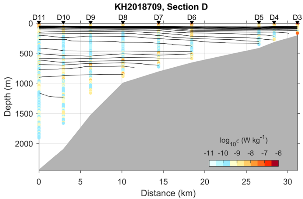
Figure 33. Distribution of dissipation rate ( \epsilon , color) and \sigma_\theta (black, CI=0.02 \text{ kg m}^{-3} ), measured by the sensors on the VMP, for Section D. \sigma_\theta is not gridded or smoothed. \epsilon is vertically averaged over 5 m. Distance is relative to the outer (deepest) station of each section.
