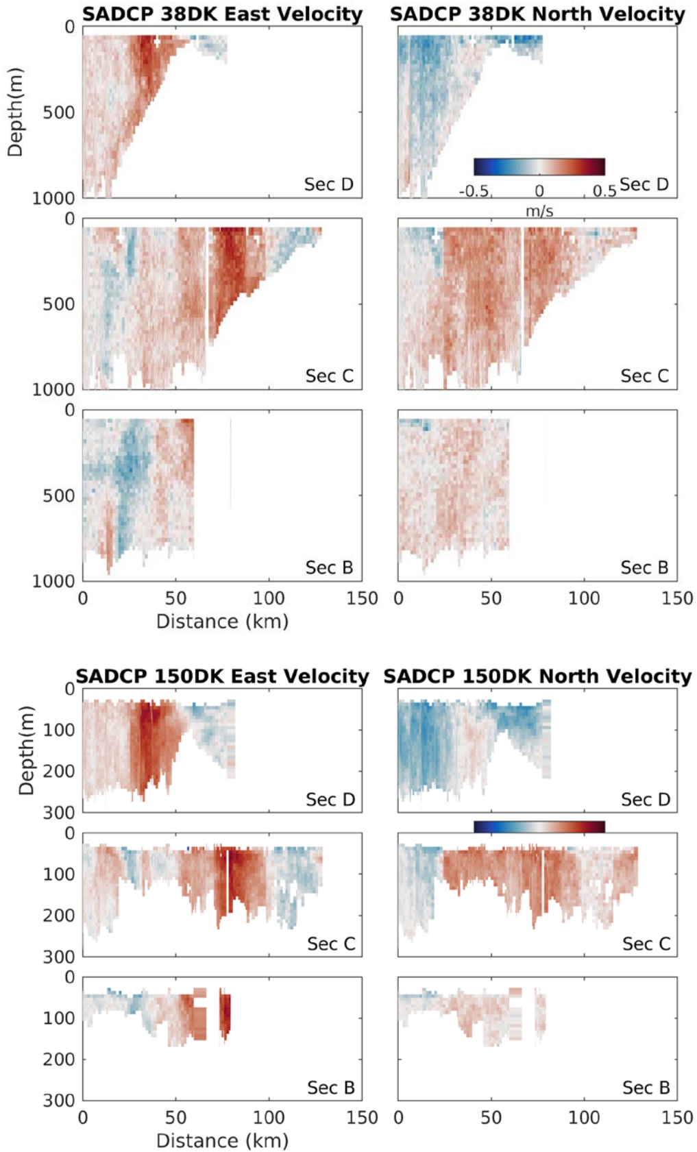
Figure 31. East and north components of the velocity measured by the SADC in Sections B, C and D, by (upper panels) the 38 kHz ADCP and (lower panels) the 150 kHz ADCP. The horizontal distance is arbitrarily referenced from deep waters toward the continental shelf on the right. Axis and color scales are identical in all panels.
