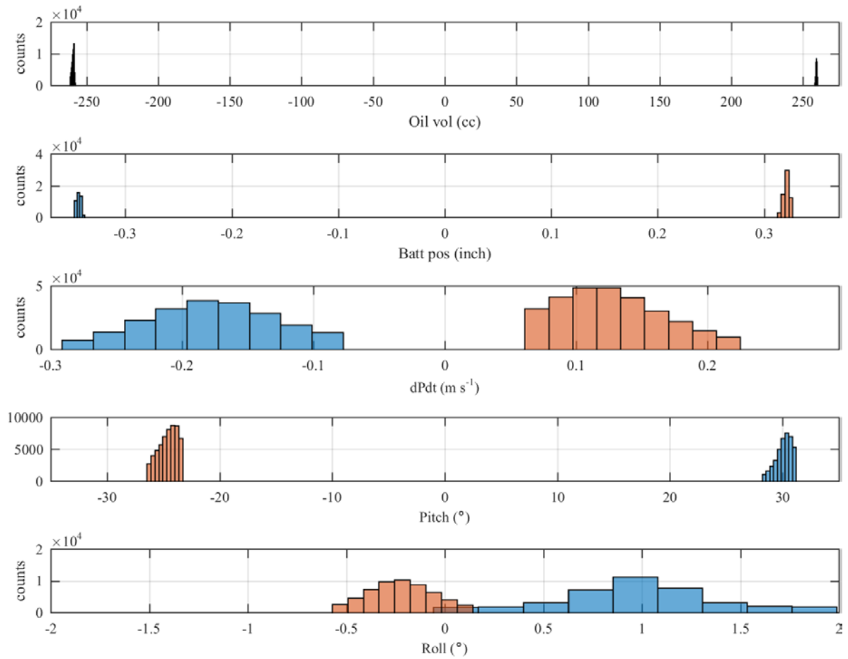
Figure 36. Histograms of (from top to bottom): pumped oil volume, battery position, vertical displacement, pitch and roll angles. Blue (resp. red) color refers to dives (resp climbs) of the glider. No data at surface or during turning points, defined as vertical displacement < 5\text{ cm/s} , are excluded.
