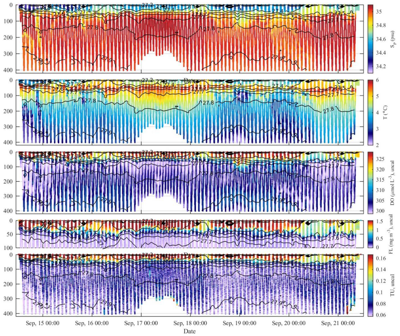
Figure 37. Depth-Time plots of (from to bottom): Practical Salinity, In situ Temperature, Dissolved Oxygen, Chlorophyll Fluorescence, Turbidity. Black lines show potential density lines.
