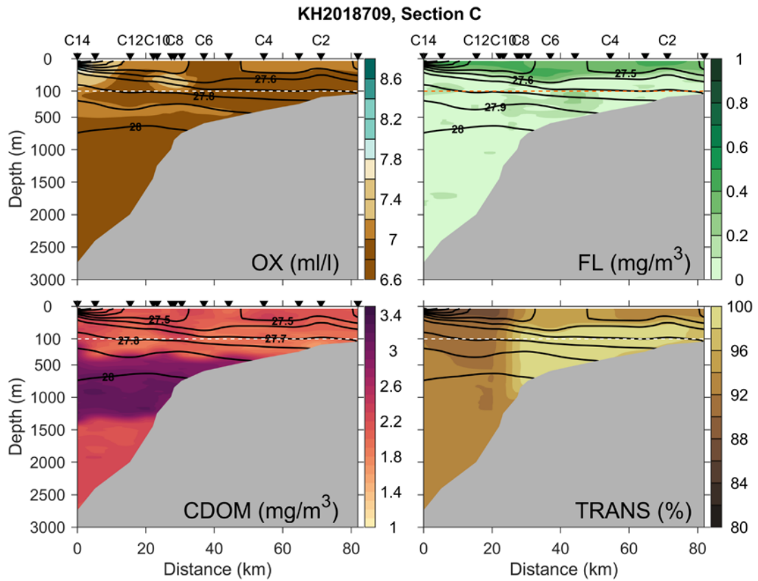
Figure 28. Contours of dissolved oxygen (OX), fluorescence (FL), CDOM and transmissivity (TRANS) for selected sections. Potential density anomaly ( \sigma_\theta ) surfaces are also shown (black). Distance is relative to the outer (deepest) station of each section. Note the change of scale at 100 m depth.
