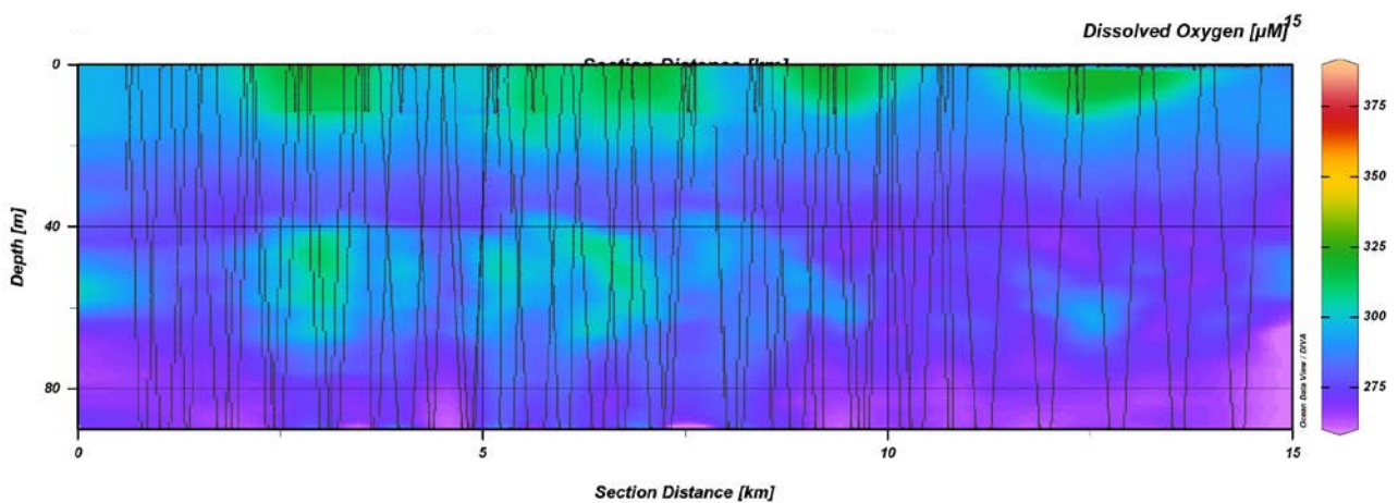
Figure 43: Dissolved oxygen profile from the TREX adaptive sampling mission. Higher values visible in the fresher and colder regions.
