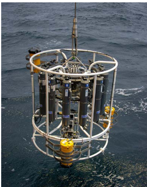
Figure 5. The CTD rosette together with the CTD sensors, 10-liter Niskin bottles, a down and uplooker ADCP, and a benthos altimeter installed. The transducers of both ADCPs and the altimeter have a non-obstructed path. The third yellow pressure case is for the LADCP batteries. The position of the lead weights and the ADCPs are adjusted to have a negligible tilt of the entire system.
