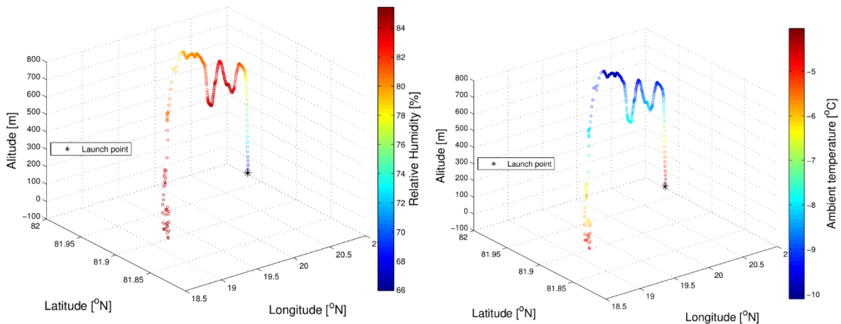
Figure 51. Measured data of relative humidity (RH) and ambient air temperature from Controlled Meteorological Balloon Olav, launched at 18 September at 13:27 UTC at 81.95N, 20.47E.
